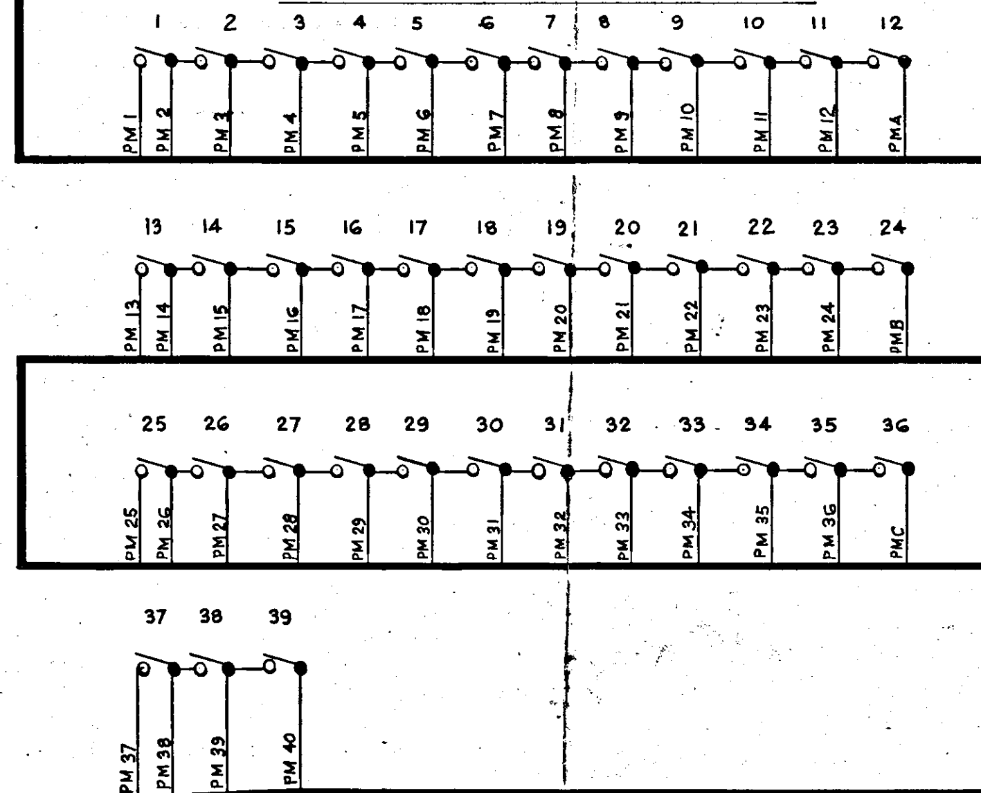
PERMANENT MAGNET PROXIMITY SWITCHES
