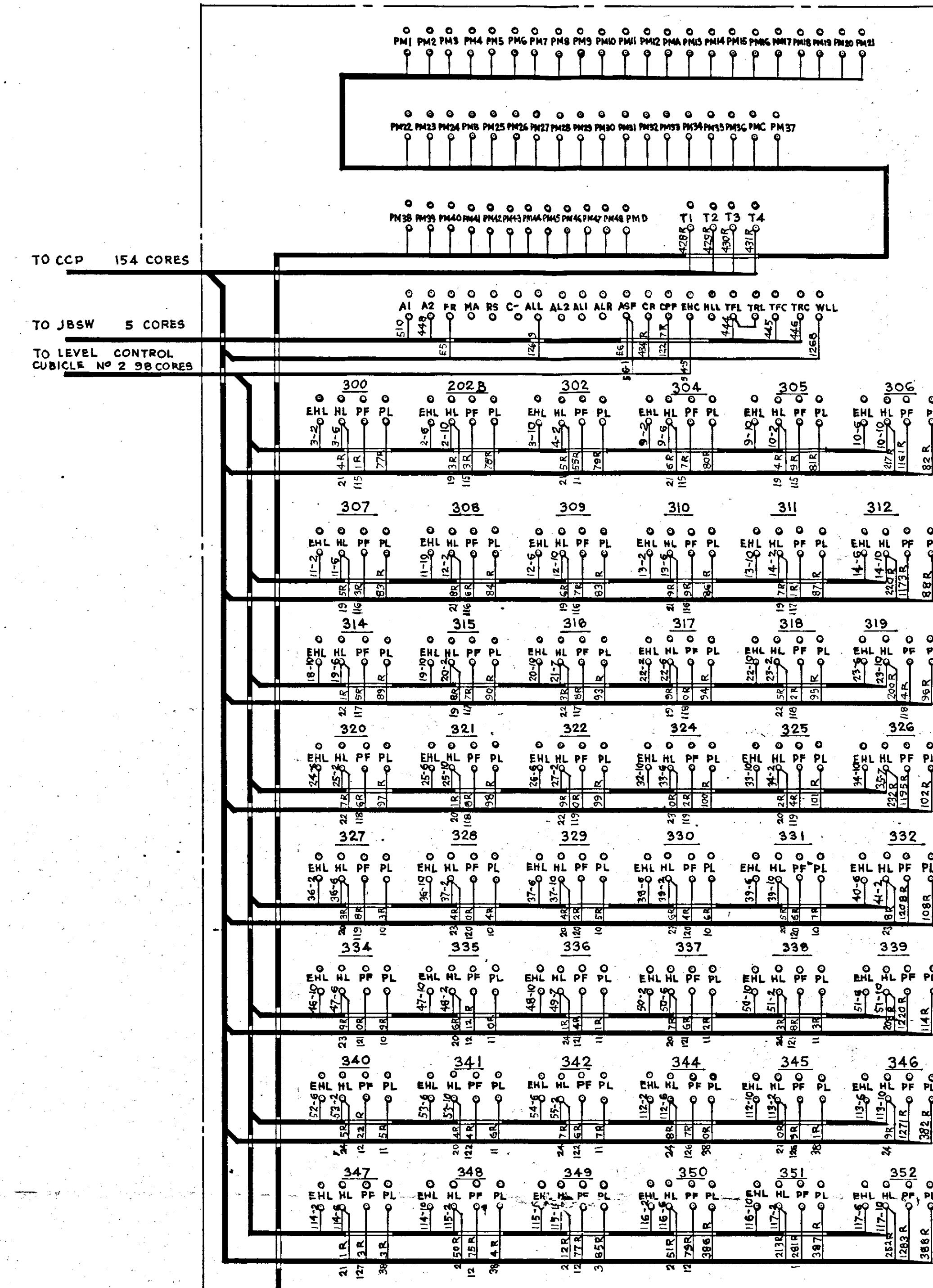
TRIPPER RELAY PANEL TRB7
