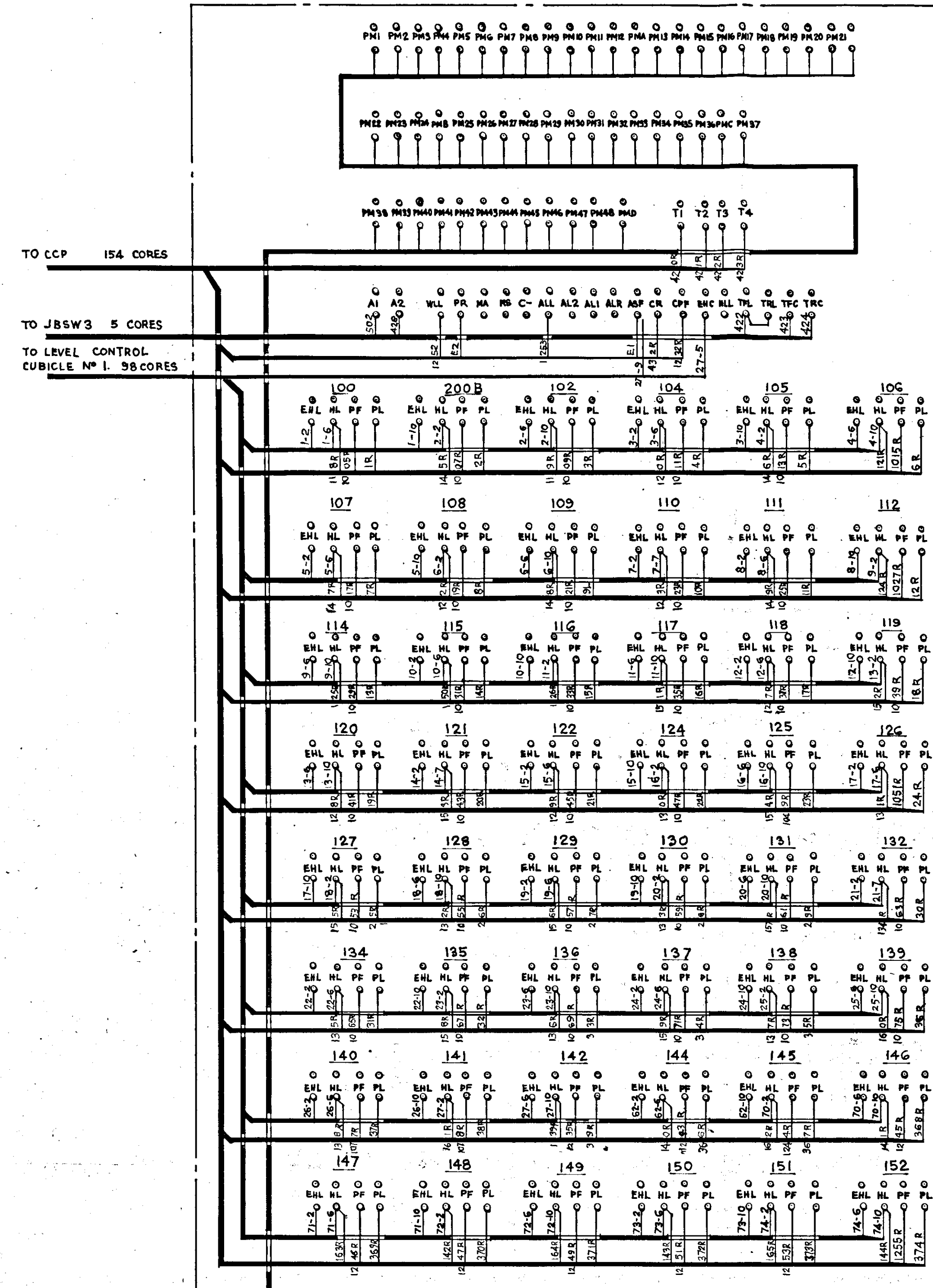
TRIPPER RELAY PANEL TRB5
